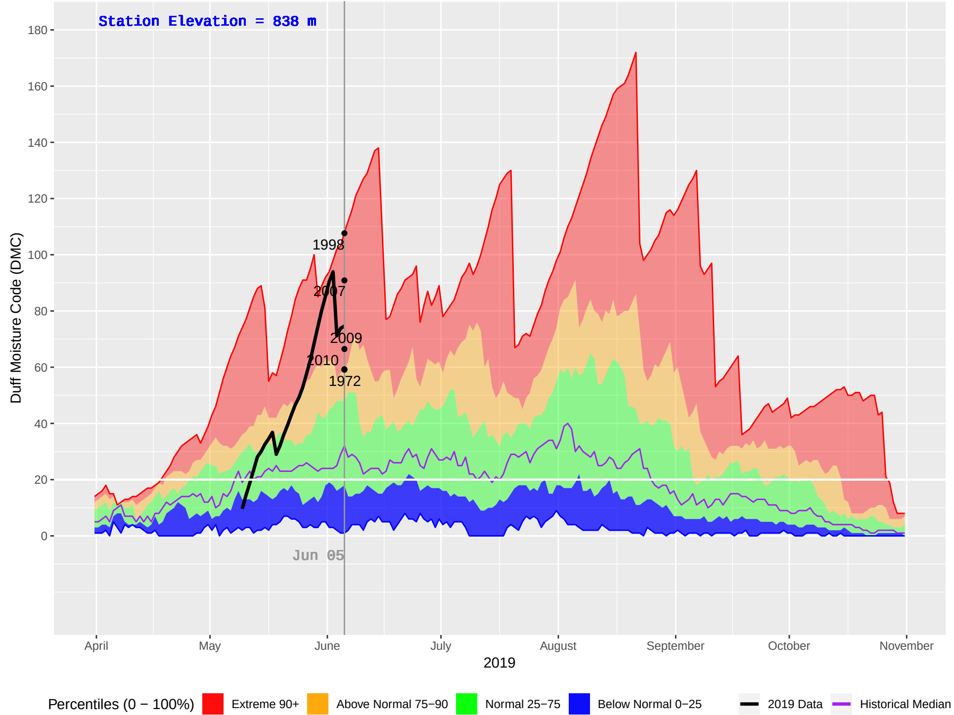
HOWARD (343) : Historical (1970–2018), Current (2019) Daily Duff Moisture Code (DMC)
