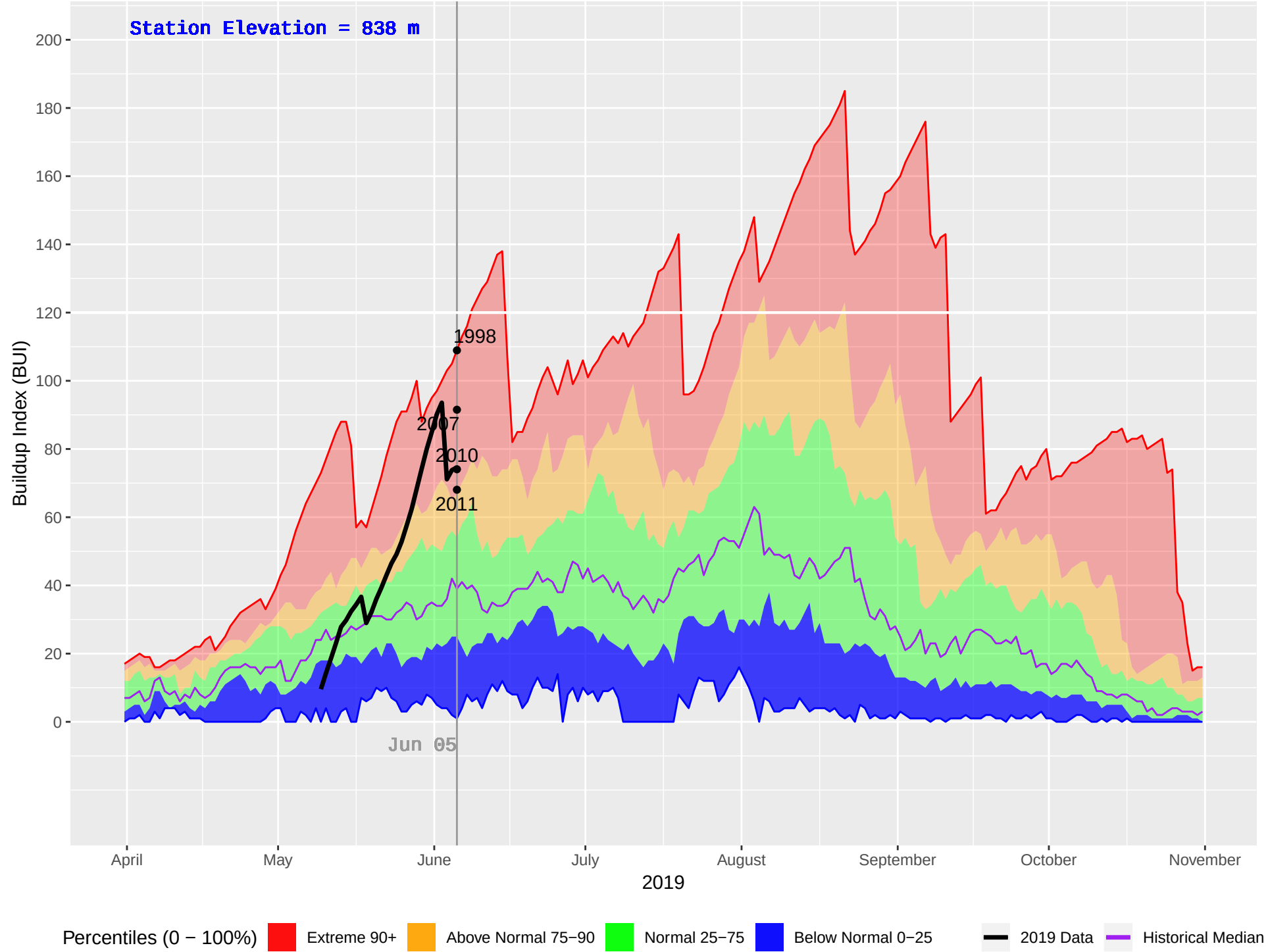
HOWARD (343) : Historical (1970–2018), Current (2019) Daily Buildup Index (BUI)
