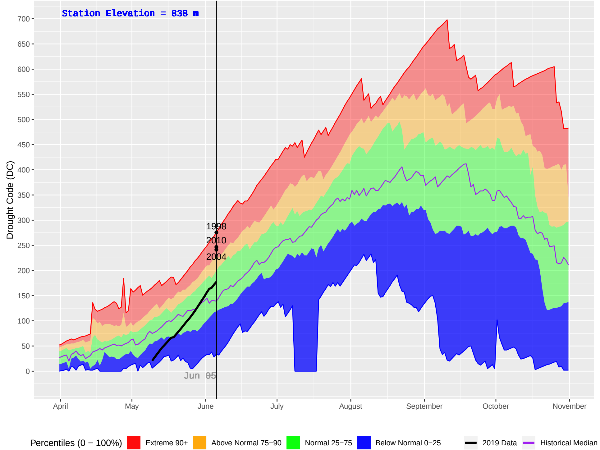
HOWARD (343) : Historical (1970–2018) and Current (2019) Daily Drought Code (DC)
