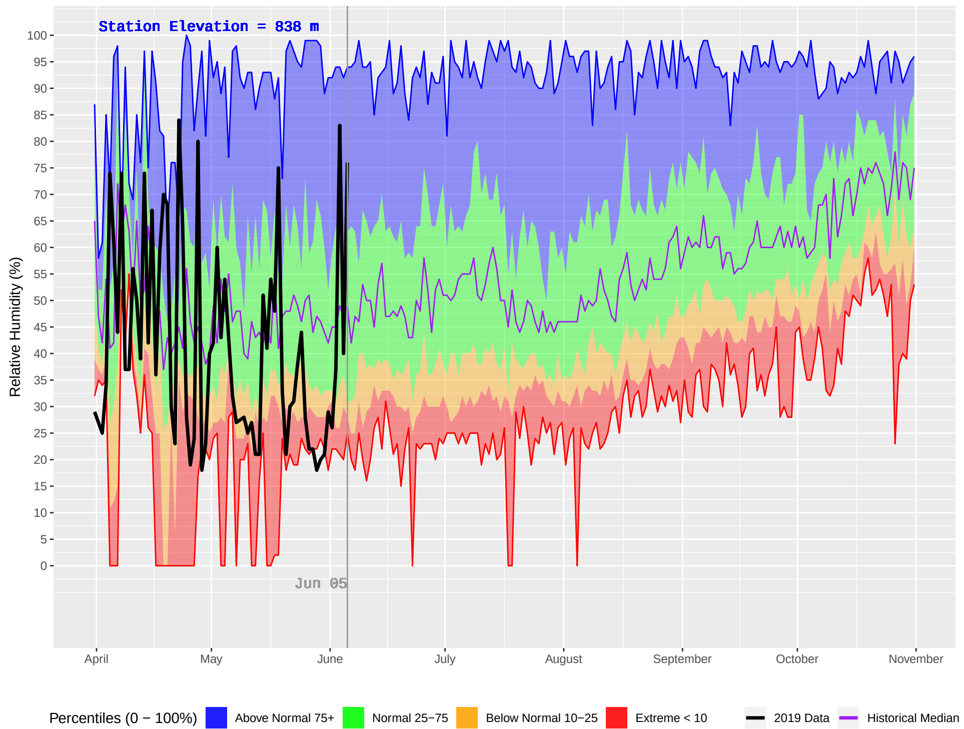
HOWARD (343) : Historical (1970–2018) and Current (2019) Daily Relative Humidity
