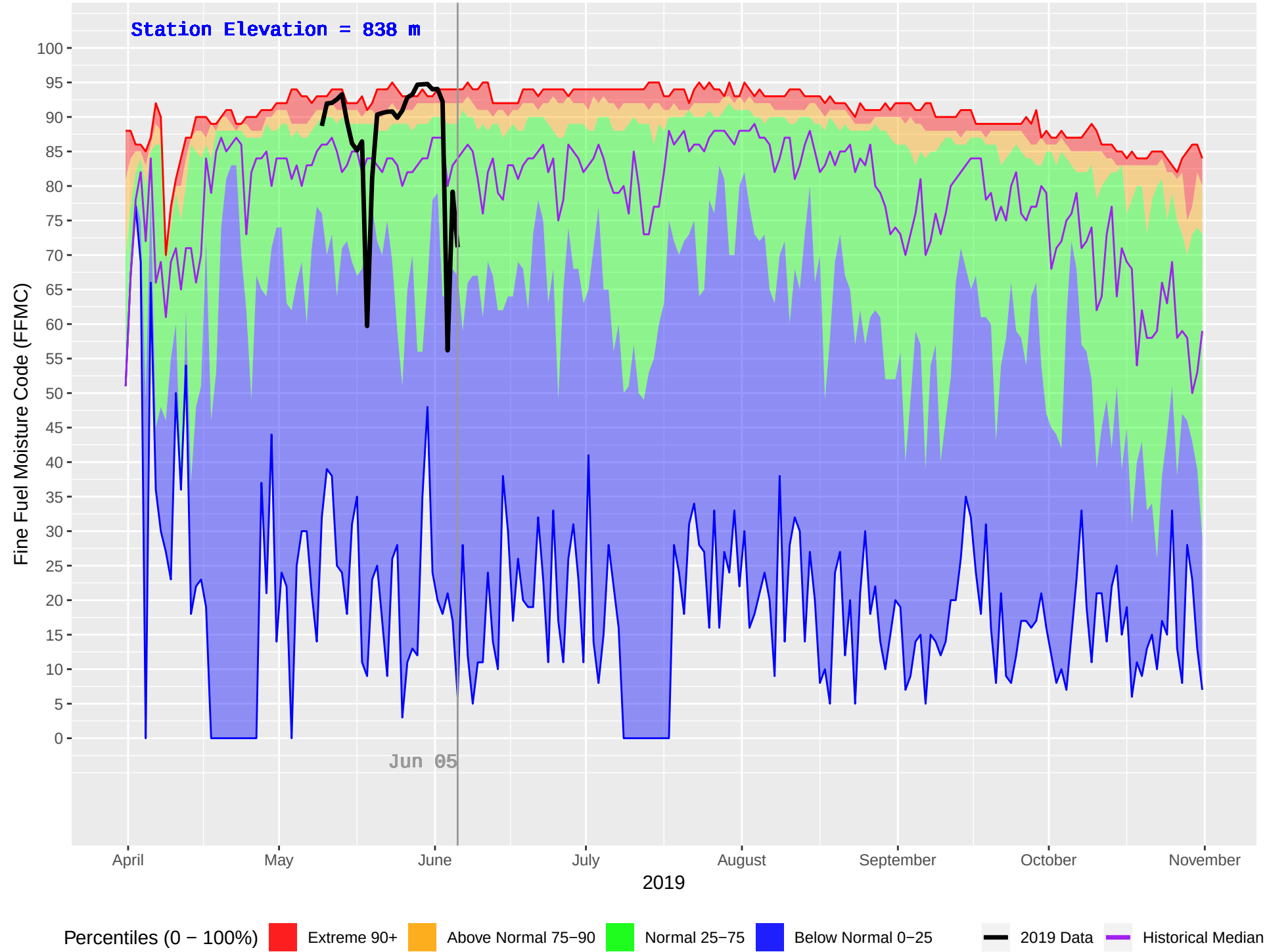
HOWARD (343) : Historical (1970–2018) and Current (2019) Daily Fine Fuel Moisture Code (FFMC)
