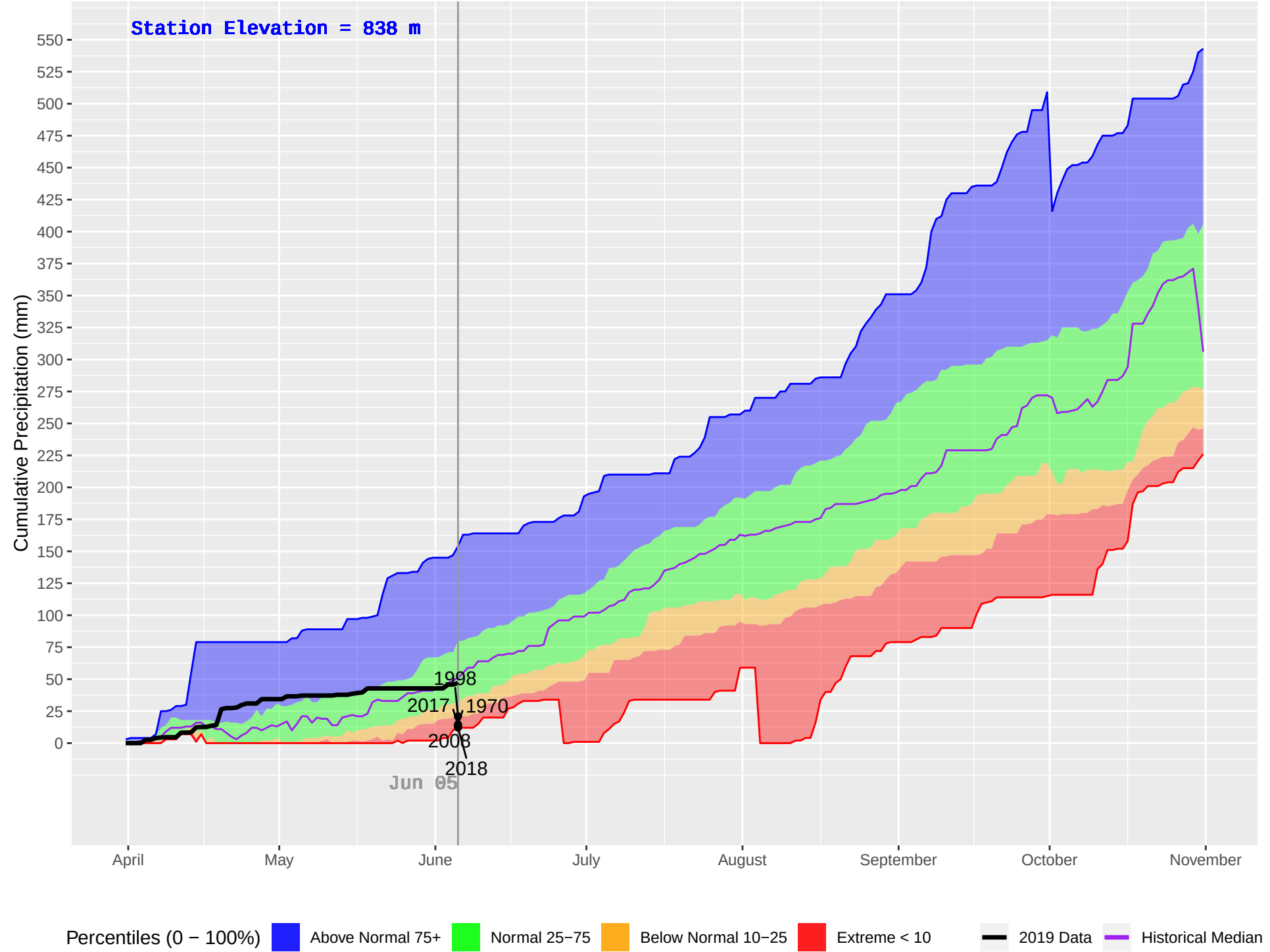
HOWARD (343) : Historical (1970–2018), Current (2019) Daily Cumulative Precipitation
